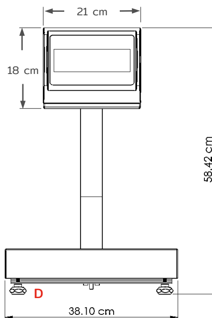
Vista frontal
